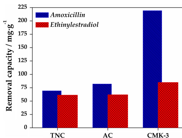
Fig. 6 Removal capacity of amoxicillin and ethinylestradiol for TNC, AC and CMK-3 samples in mg/g
